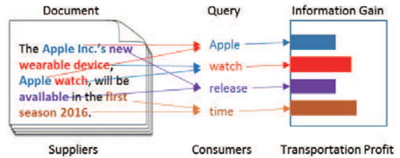
Figure 1: Semantic Matching as Word Transportation.
